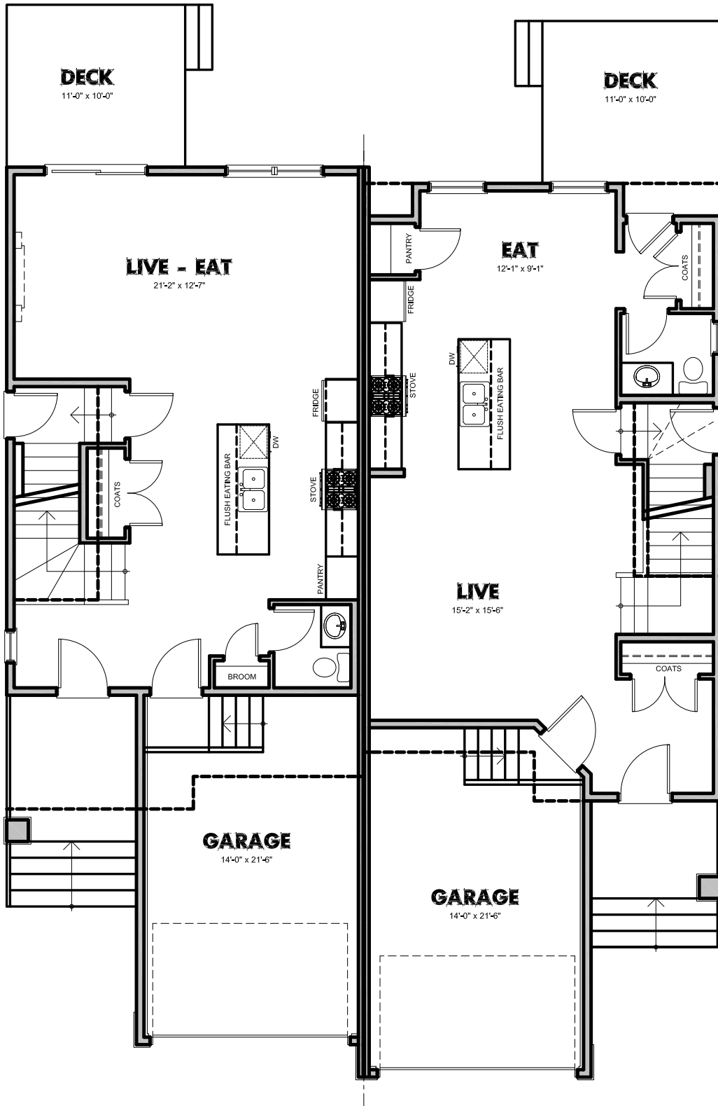
MAIN FLOOR PLAN UNIT 20/24 715 / 762SQ.FT.
